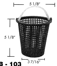
B - 103 Jacuzzi 16-0470 P-21 [Tapered] (Plastic)
