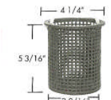
B - 187 (Plastic) Swimaquip 16200-9 XL6 [short] See B-44
