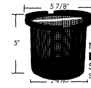
B - 37 American Concrete Skimmer #850001 - S-10 Skimmer Basket (Plastic) *See B-28 for Plastic Coated
