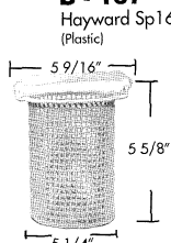
B - 176 Marlow 25774-00 (Plastic)
