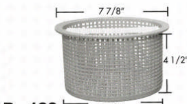
B - 183 Jacuzzi 43-0507-07 Skimmer Basket (Plastic) Same as B-113 Metal
