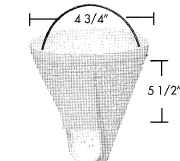
B - 177 American Products 393004 Noryl Basket (Plastic Coated)
